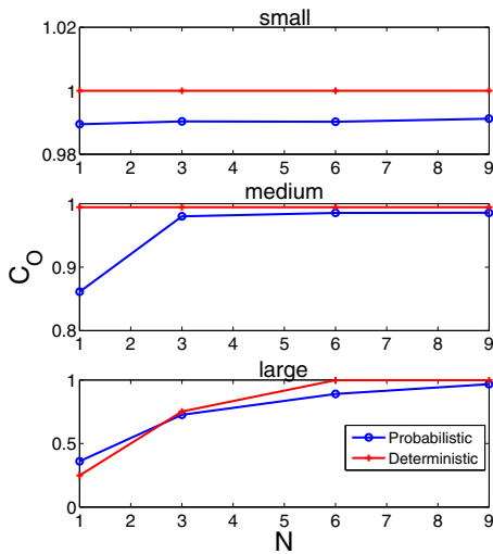
Fig. 3. Observation area coverage versus number of UAVs
