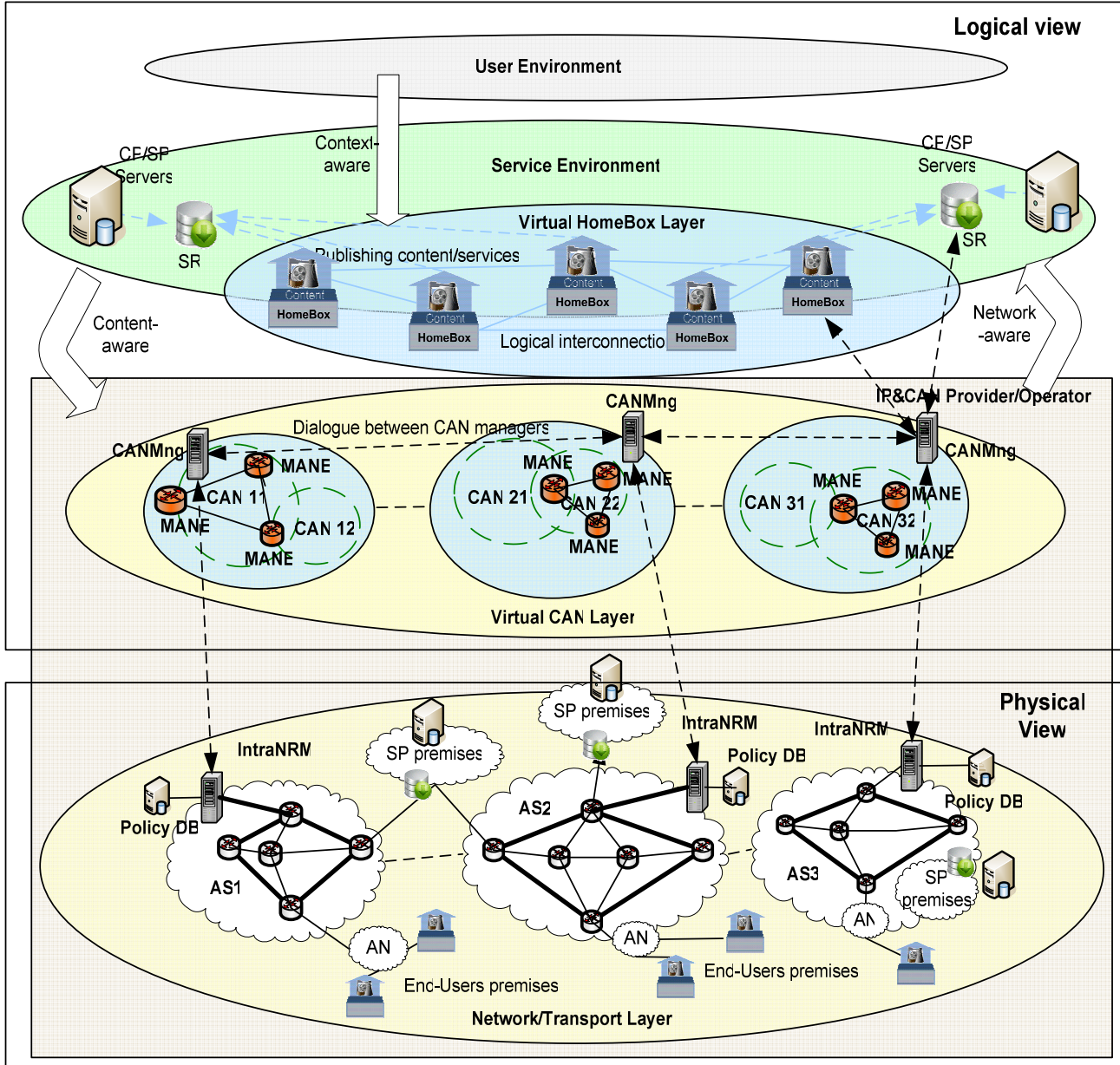
Figure 1 The ALICANTE Architecture: details on Virtual CAN Layer
