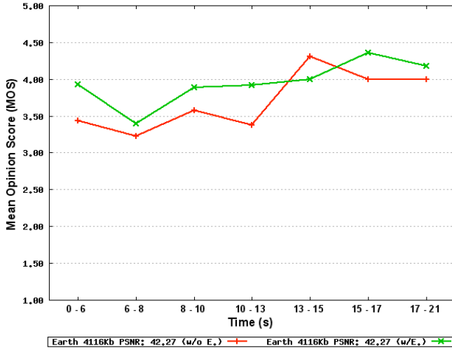
Figure 7. Continuous MOS for Earth at 4 Mbit/s.
