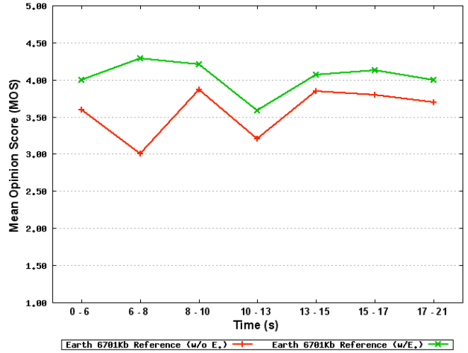
Figure 8. Continuous MOS for Earth at 6 Mbit/s.
