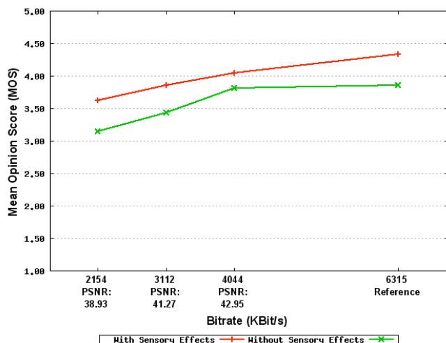
Figure 9. MOS vs. PSNR/bit-rate for Babylon A.D.
