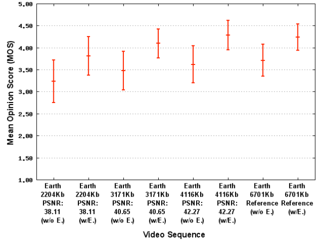
Figure 6. MOS and confidence interval for Earth.
