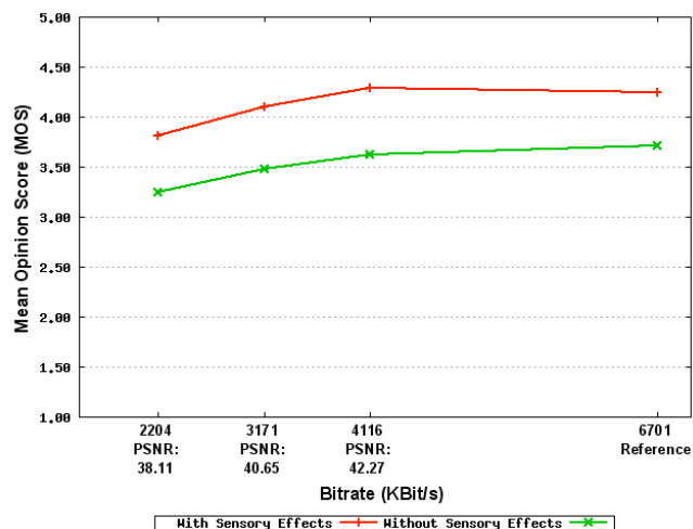
Figure 10. MOS vs. PSNR/bit-rate for Earth.
